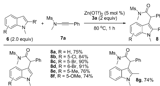
Scheme 2. Intermolecular reaction of the indoles 6 with the ynamide 7a through oxidative zinc catalysis.
