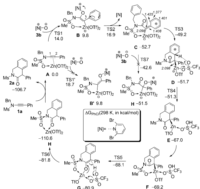
Scheme 4. Plausible mechanism. Theoretical investigations on the reaction pathways for the formation of 2a : relative free energies ( \Delta G_{\text{PhCl}} , in \text{kcal mol}^{-1} ) of key intermediates and transition states were computed at the M06/6-31G(d,p)/LanL2DZ level of theory in PhCl at 298 K.
