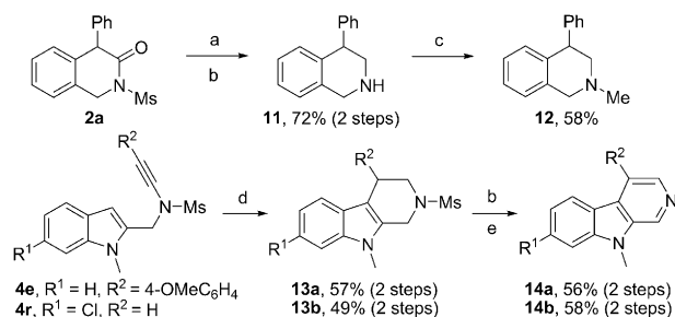
Scheme 3. Synthetic applications. Reagents and conditions: a) \text{B}_2\text{H}_6 \cdot \text{THF} (4 equiv), THF, reflux; b) Red-Al (5 equiv), toluene, 110 °C; c) HCHO, NaBH 4 , MeOH, RT; d) \text{Zn}(\text{OTf})_2 (5 mol %), 3a (2.0 equiv), DCE, 80 °C, 1 h; \text{B}_2\text{H}_6 \cdot \text{THF} (4 equiv), THF, reflux, 6 h; e) for 13a : Pd/C, p -xylene, 135 °C; for 13b : MnO 2 (2 equiv), toluene, 100 °C. THF = tetrahydrofuran.
